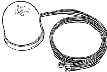
4) LTE antenna 2 x 4G LTE/3G/2G MIMO Ground Plane Dependent IP67 IK09 IP69K Antenna
